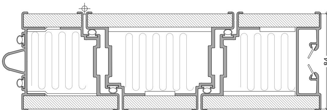
Option with door leaf in panel
