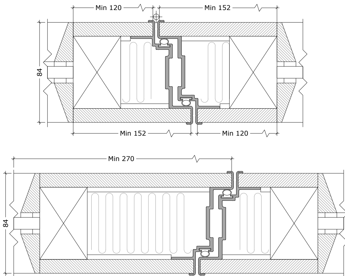
Option with door leaf in panel
